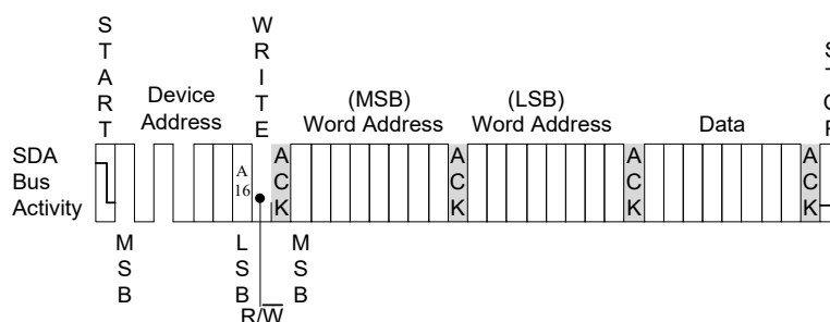
Figure 6. Byte Write
