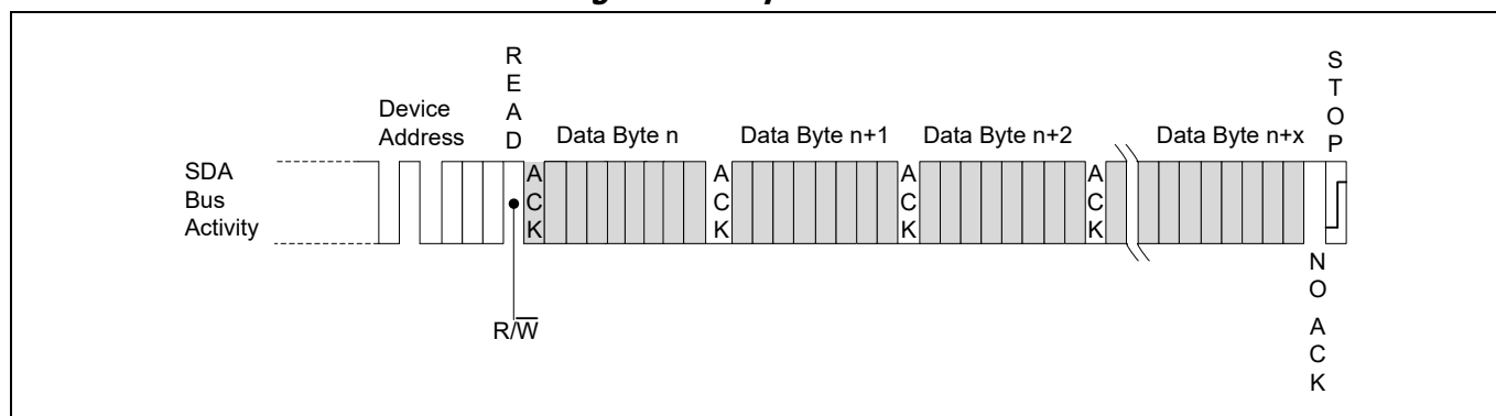
Figure 10. Sequential Read
