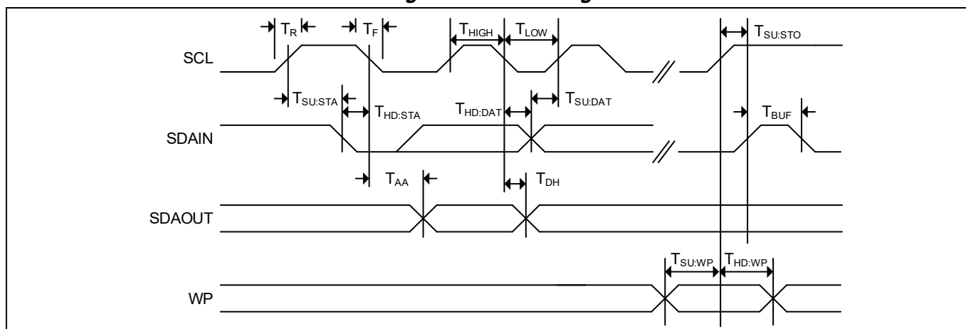
Figure 11. Bus Timing
