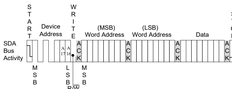
Figure 6. Byte Write
