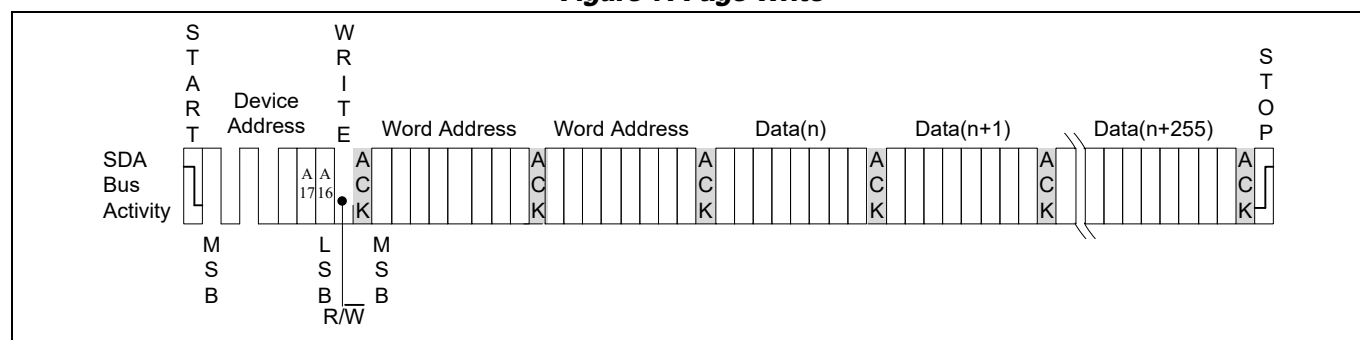
Figure 7. Page Write
