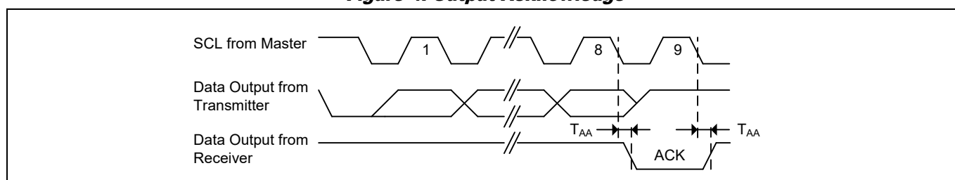
Figure 4. Output Acknowledge
