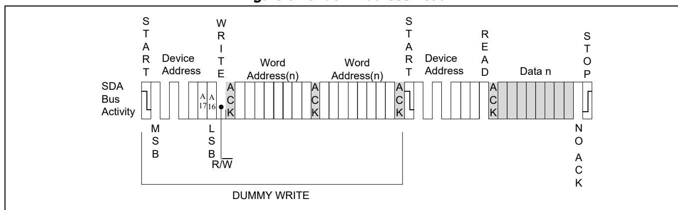
Figure 9 Random Address Read
