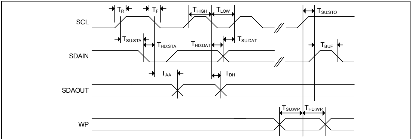
Figure 11. Bus Timing
