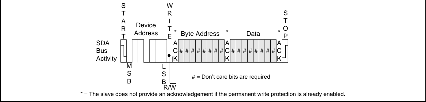
Figure 7.7 Set PSWP
