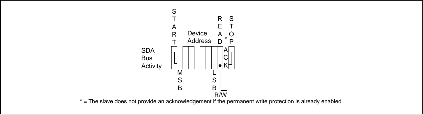
Figure 7.8 Read PSWP
