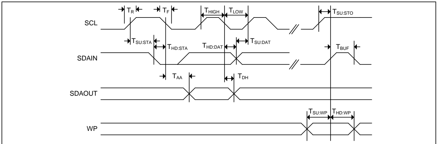
Figure 5-6. Bus Timing
