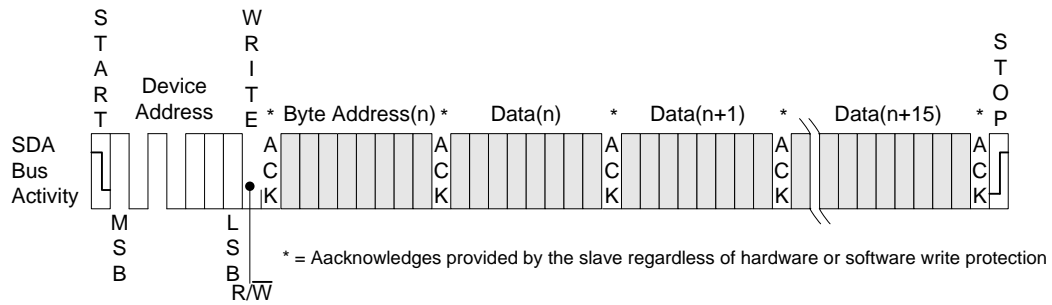
Figure 7.3 Page Write
