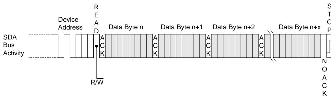
Figure 7.6 Sequential Read
