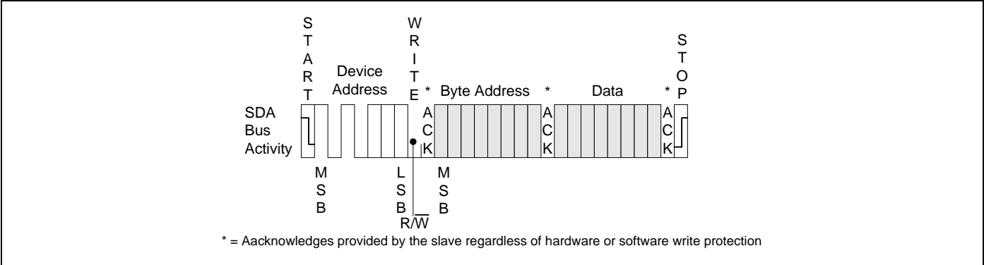
Figure 7.2 Byte Write
